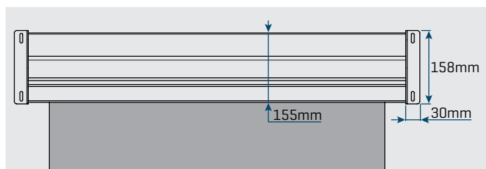
CURTAIN WITH SAFE PROFILE
