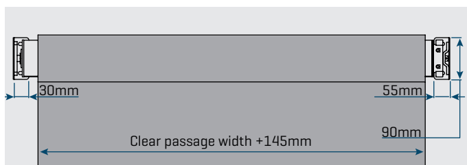
CURTAIN WITHOUT SAFE PROFILE
